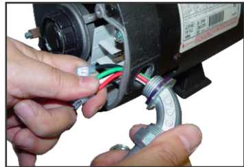
3) Route the power wires through the conduit hole and pull toward you to allow for the cord assy to be rotated for tightening.
